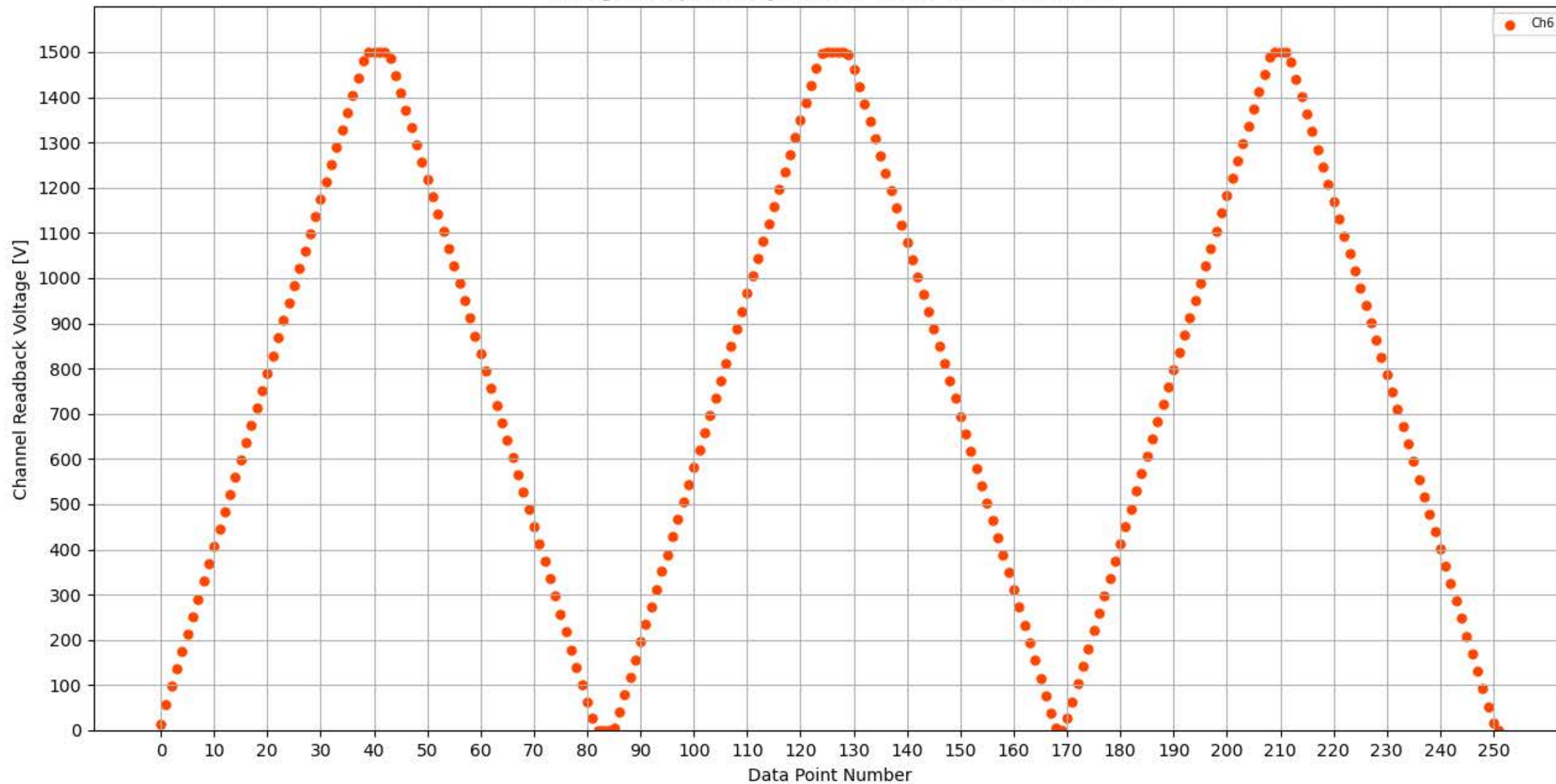
Voltage Ramp Test (Python) Bd #350, Slot #13, Ch #6
