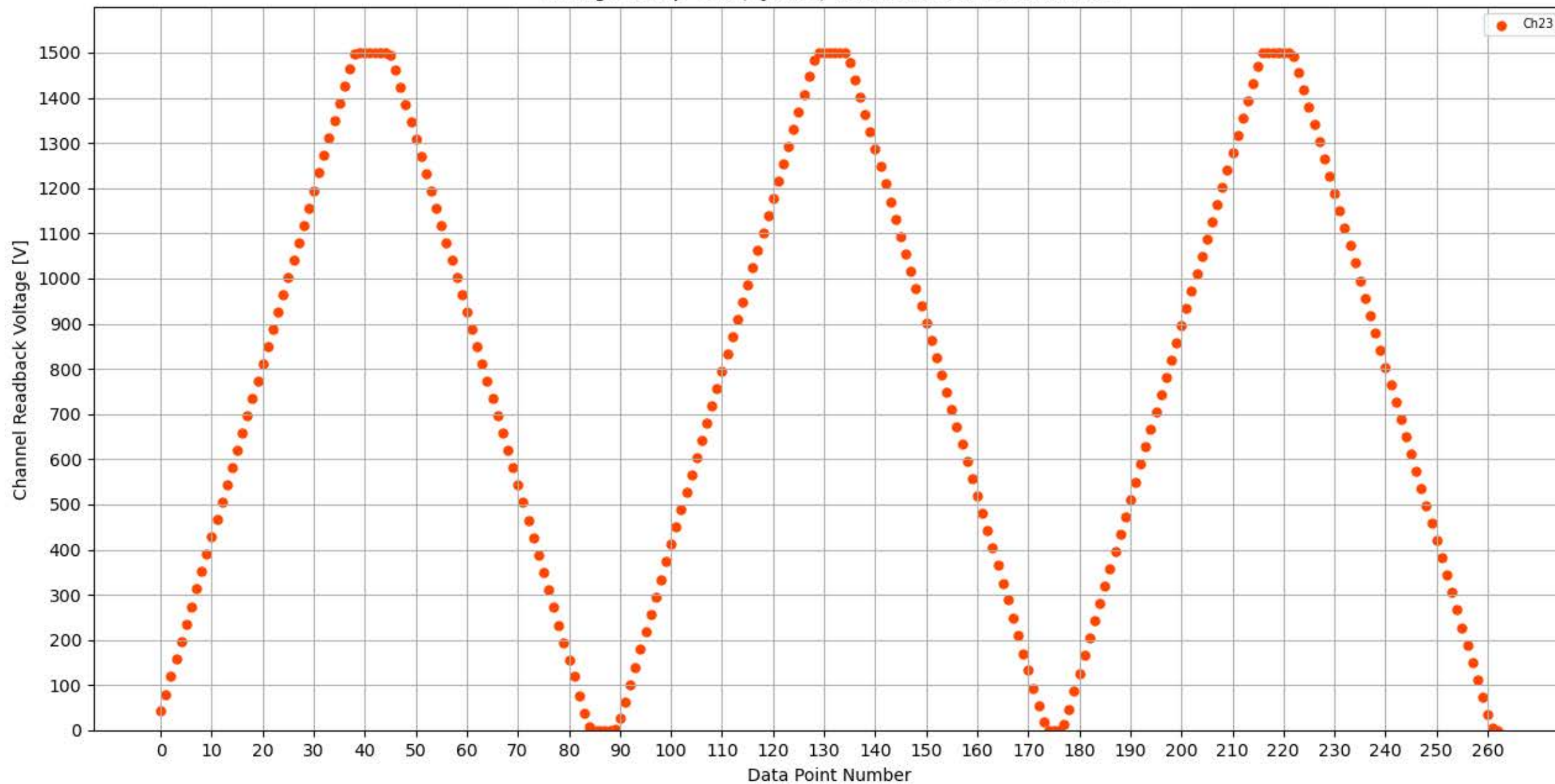
Voltage Ramp Test (Python) Bd #350, Slot #13, Ch #23
