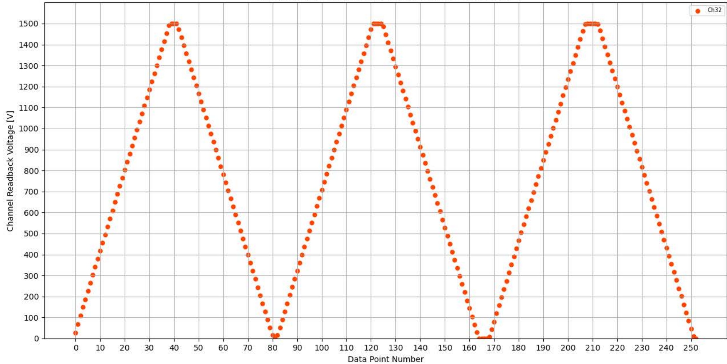
Voltage Ramp Test (Python) Bd #350, Slot #13, Ch #32
