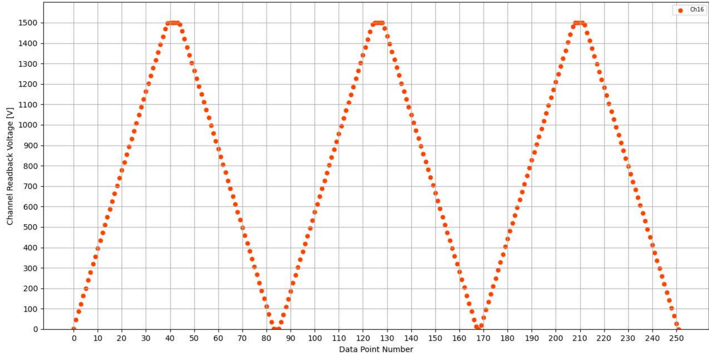
Voltage Ramp Test (Python) Bd #350, Slot #13, Ch #16
