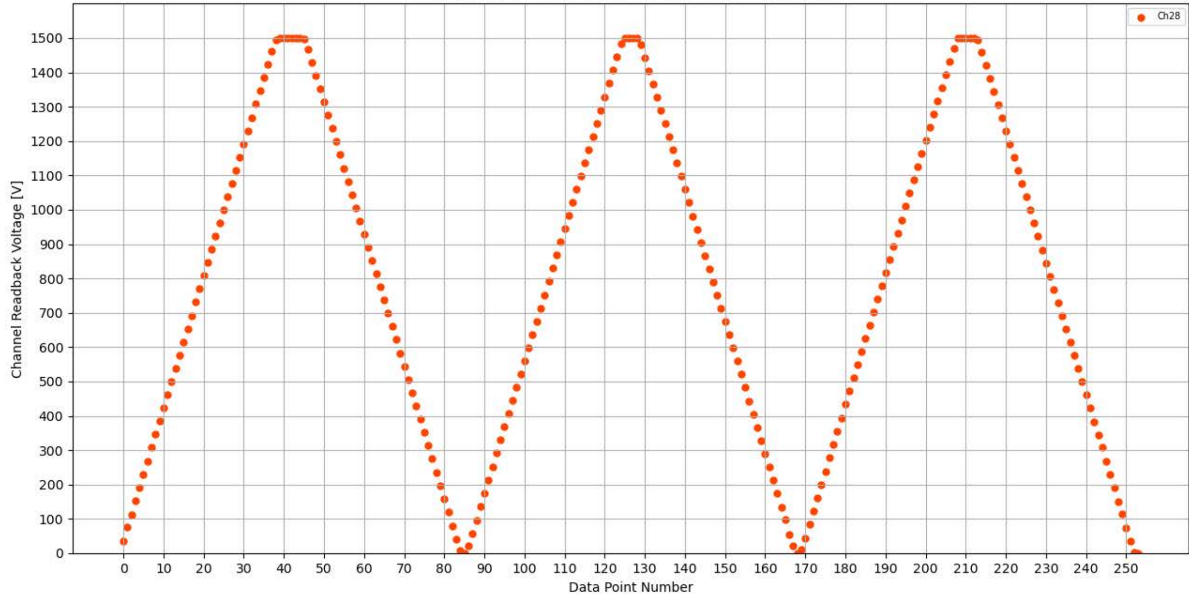
Voltage Ramp Test (Python) Bd #350, Slot #13, Ch #28
