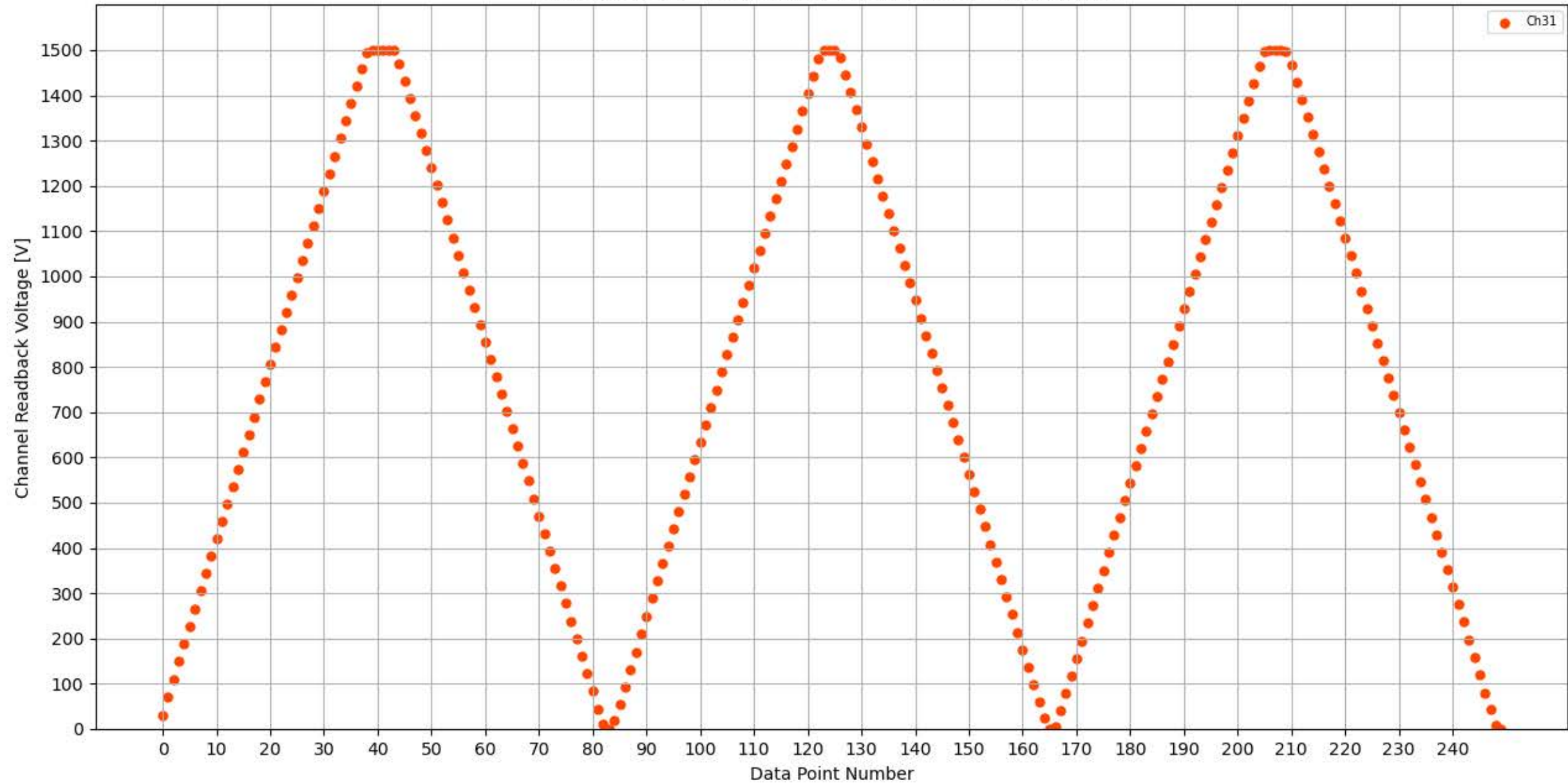
Voltage Ramp Test (Python) Bd #350, Slot #13, Ch #31
