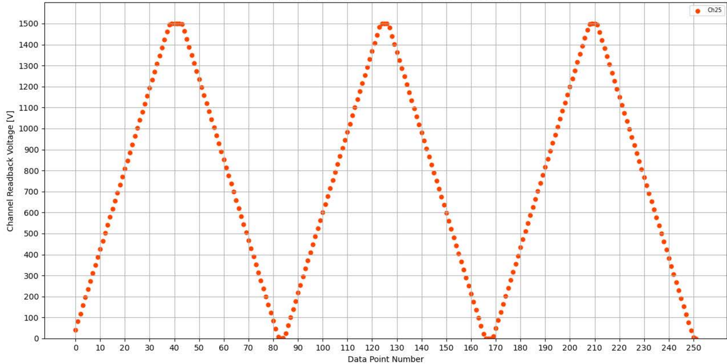
Voltage Ramp Test (Python) Bd #350, Slot #13, Ch #25
