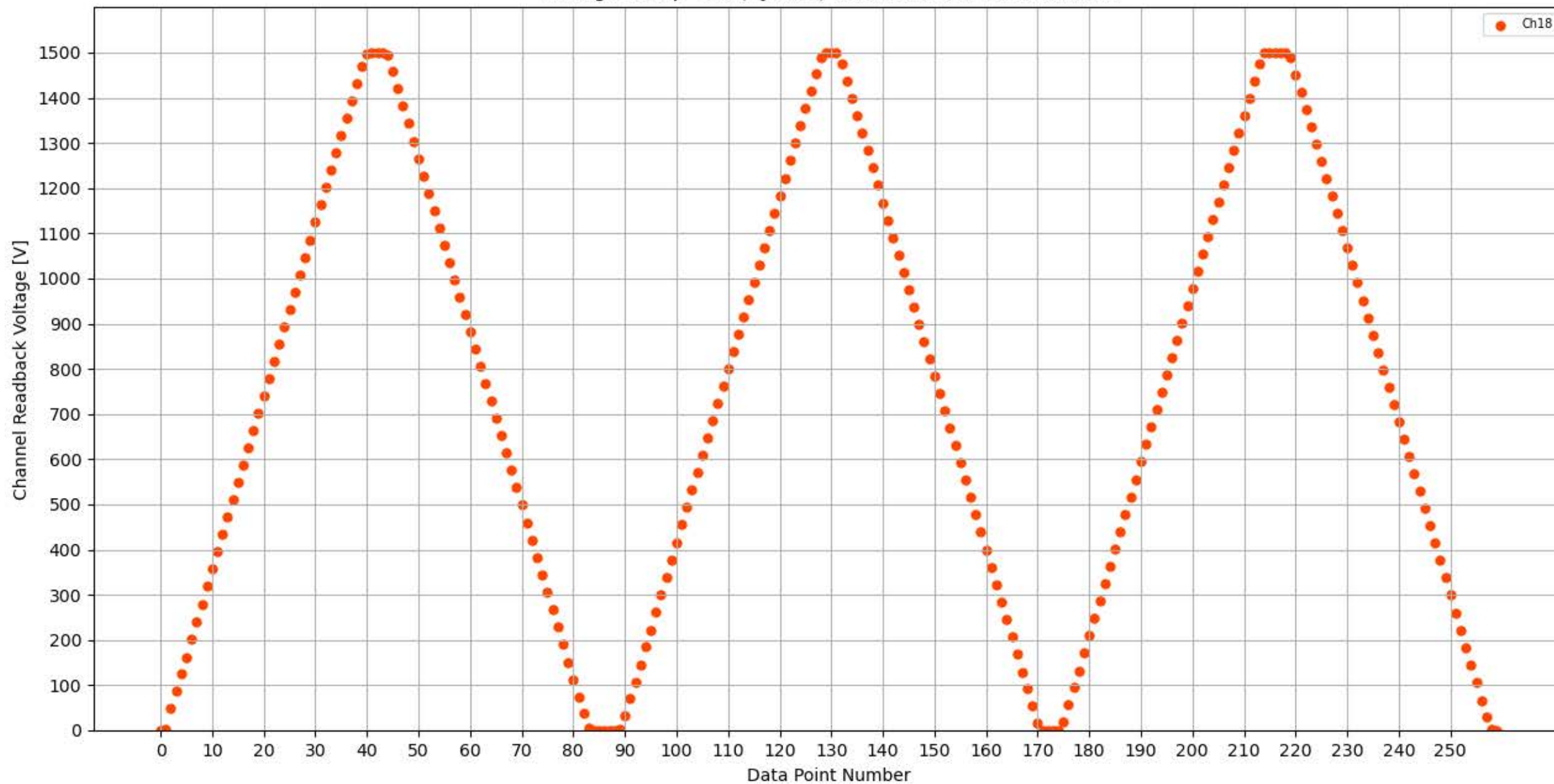
Voltage Ramp Test (Python) Bd #350, Slot #13, Ch #18
