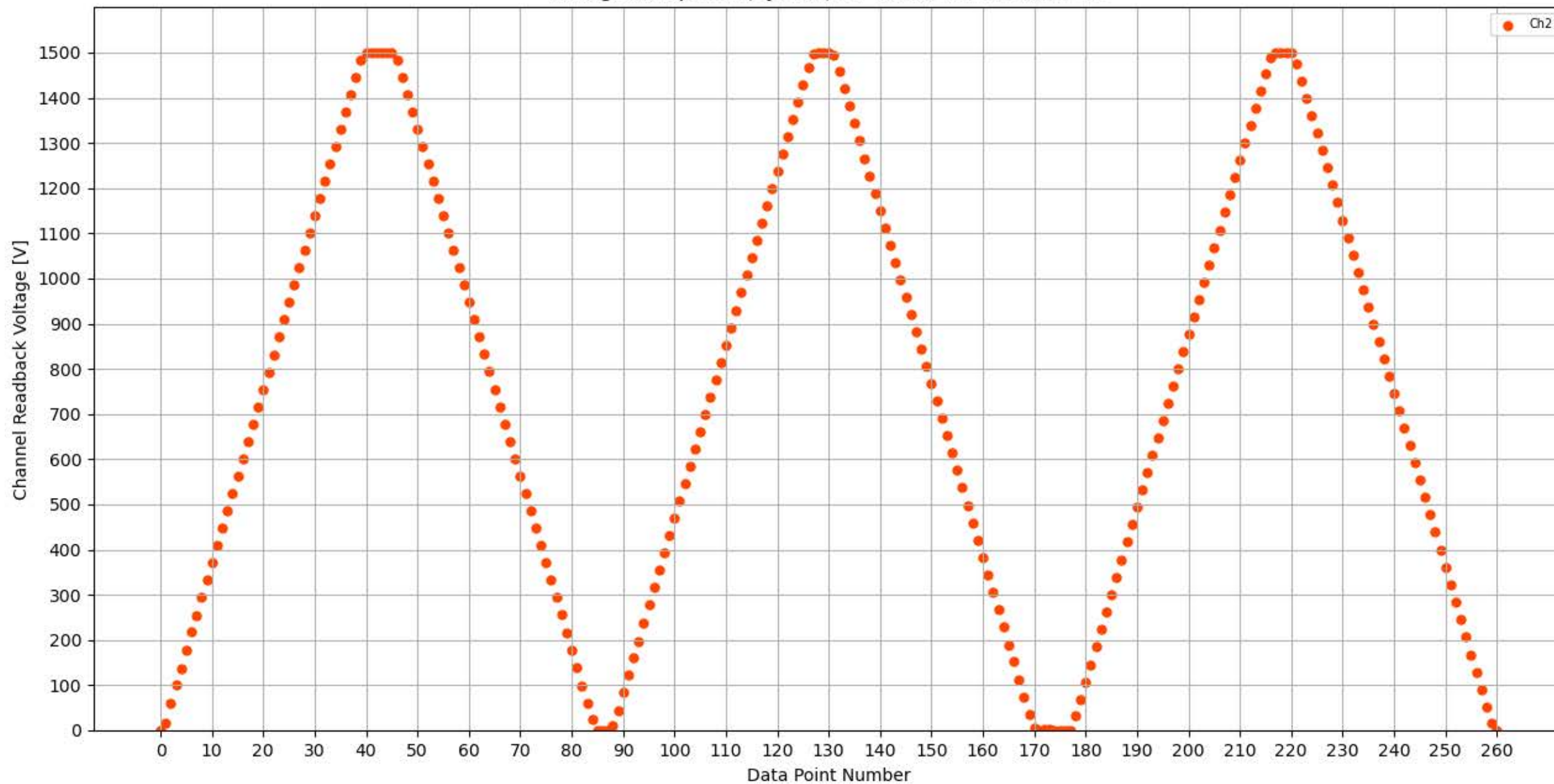
Voltage Ramp Test (Python) Bd #350, Slot #13, Ch #2
