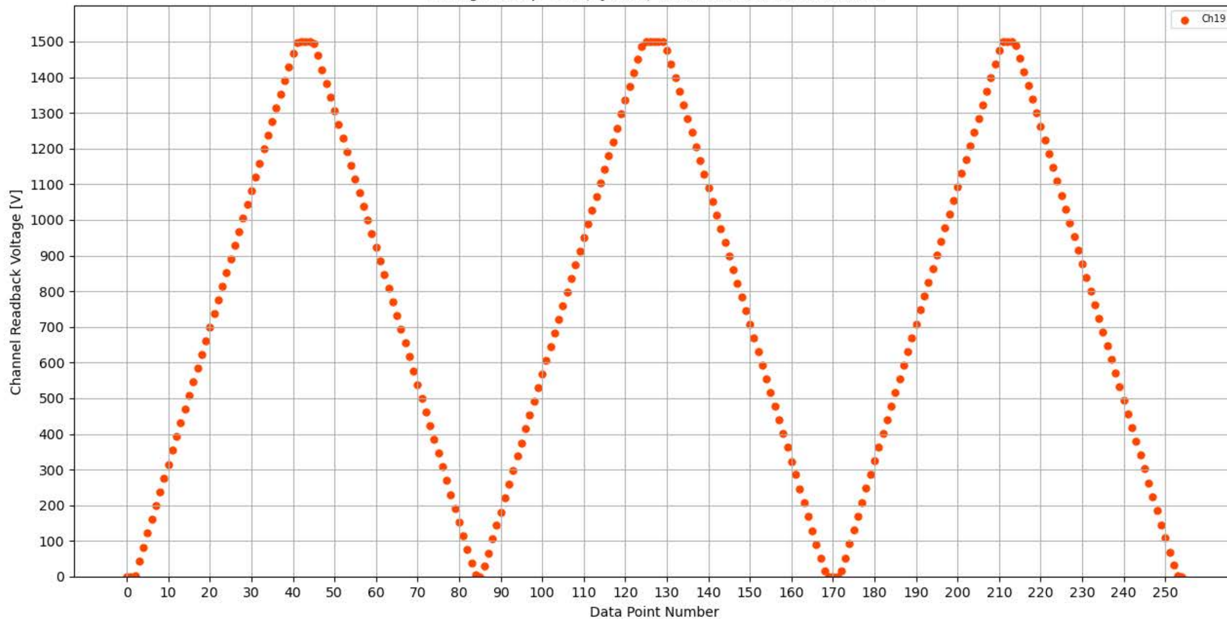
Voltage Ramp Test (Python) Bd #350, Slot #13, Ch #19
