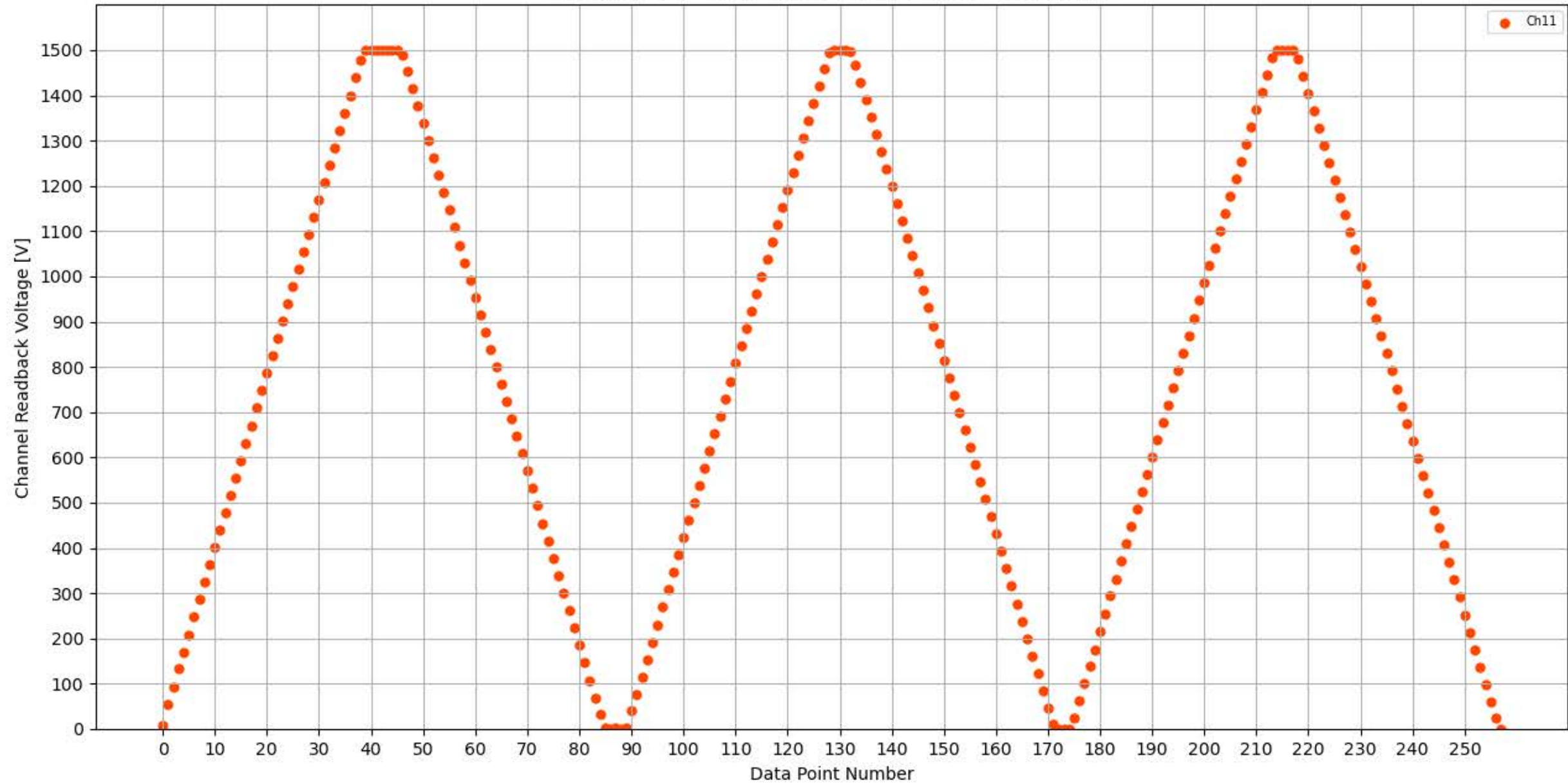
Voltage Ramp Test (Python) Bd #350, Slot #13, Ch #11
