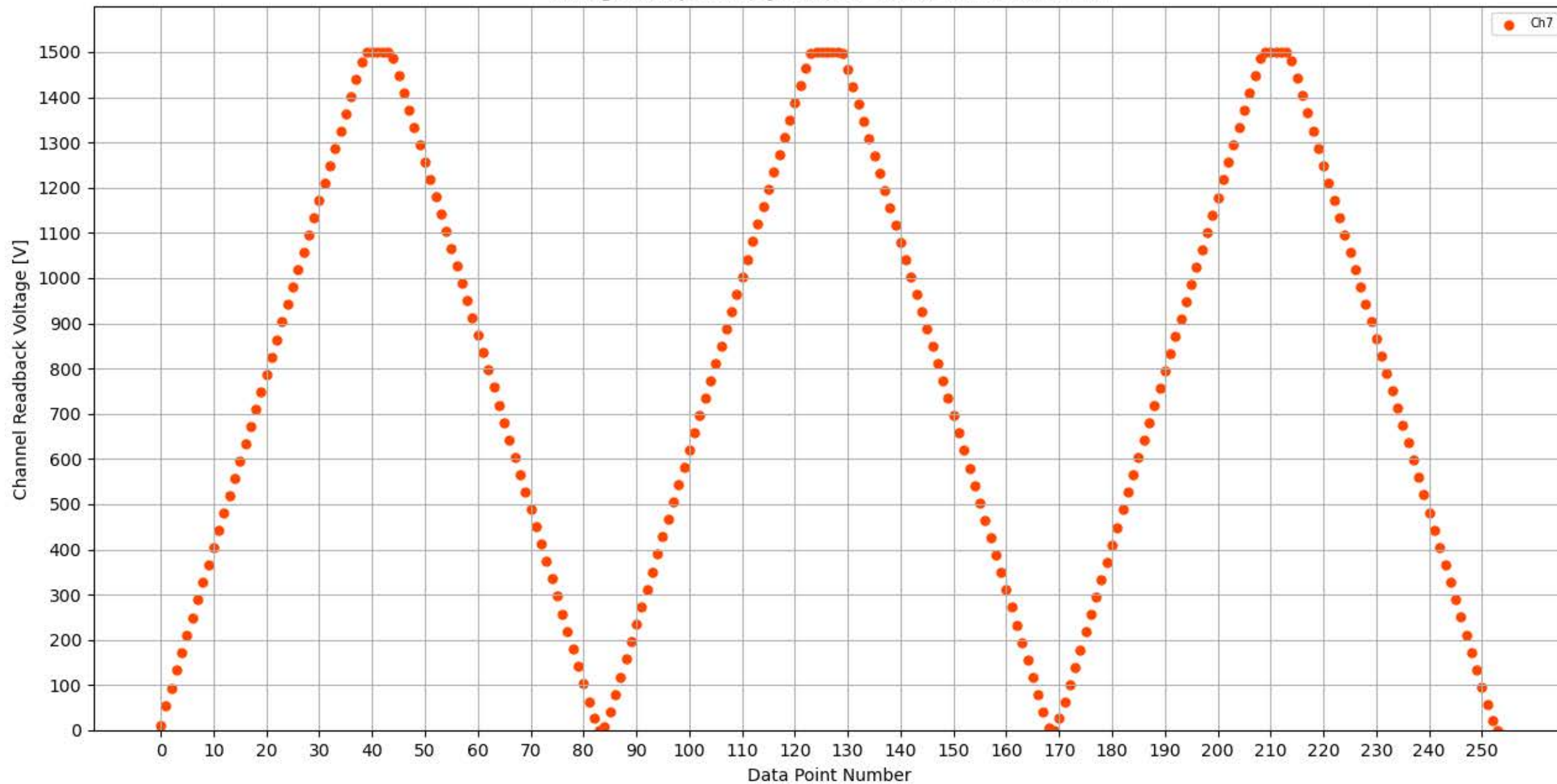
Voltage Ramp Test (Python) Bd #350, Slot #13, Ch #7
