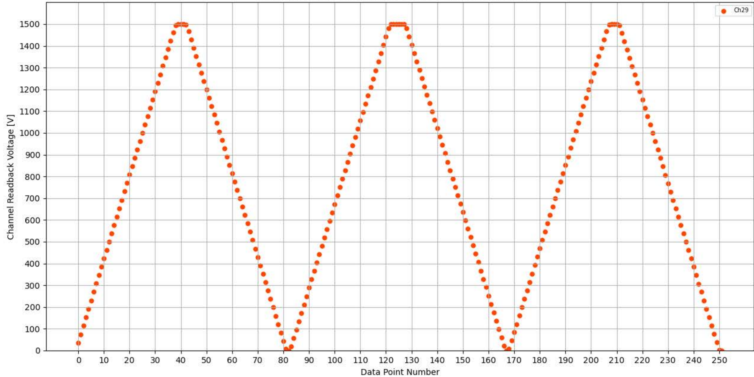
Voltage Ramp Test (Python) Bd #350, Slot #13, Ch #29
