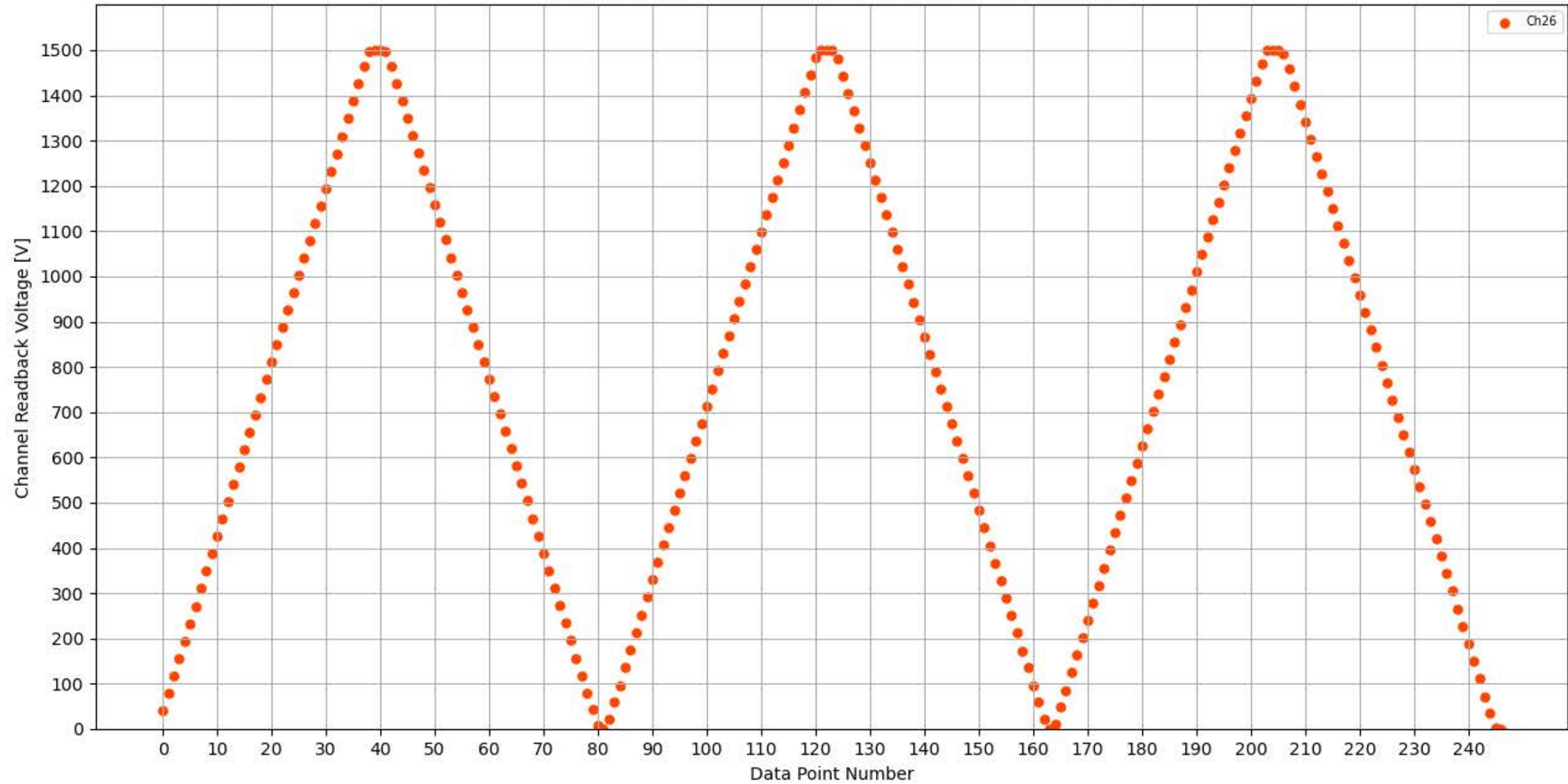
Voltage Ramp Test (Python) Bd #350, Slot #13, Ch #26
