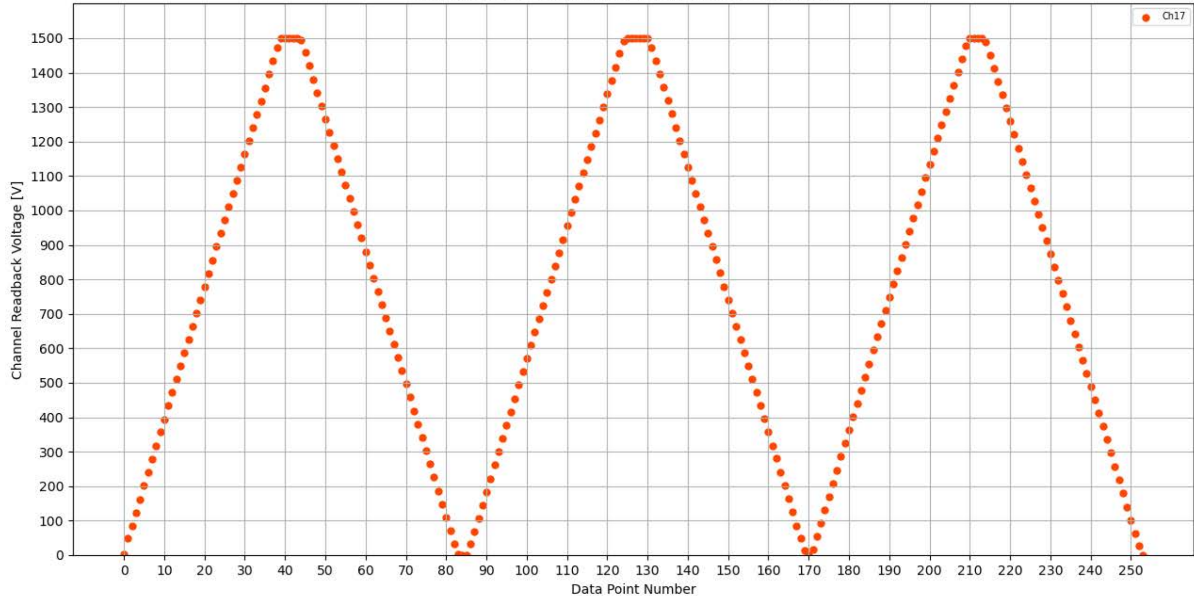
Voltage Ramp Test (Python) Bd #350, Slot #13, Ch #17
