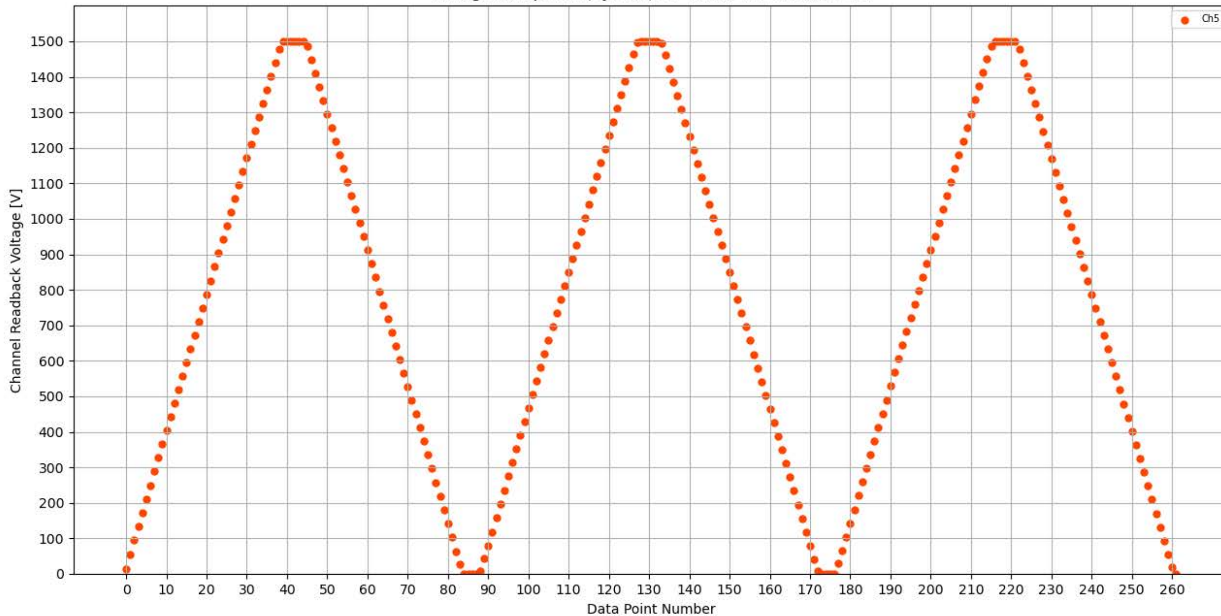
Voltage Ramp Test (Python) Bd #350, Slot #13, Ch #5
