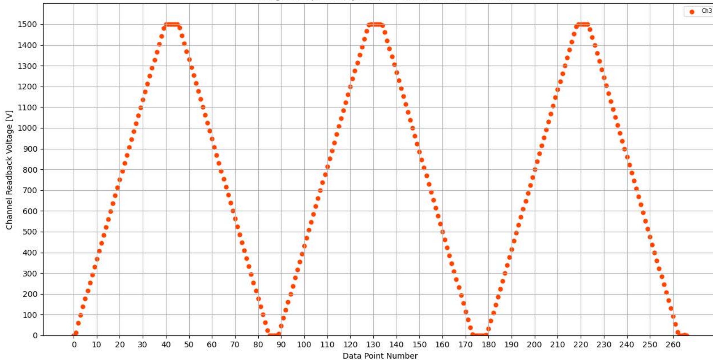
Voltage Ramp Test (Python) Bd #350, Slot #13, Ch #3
