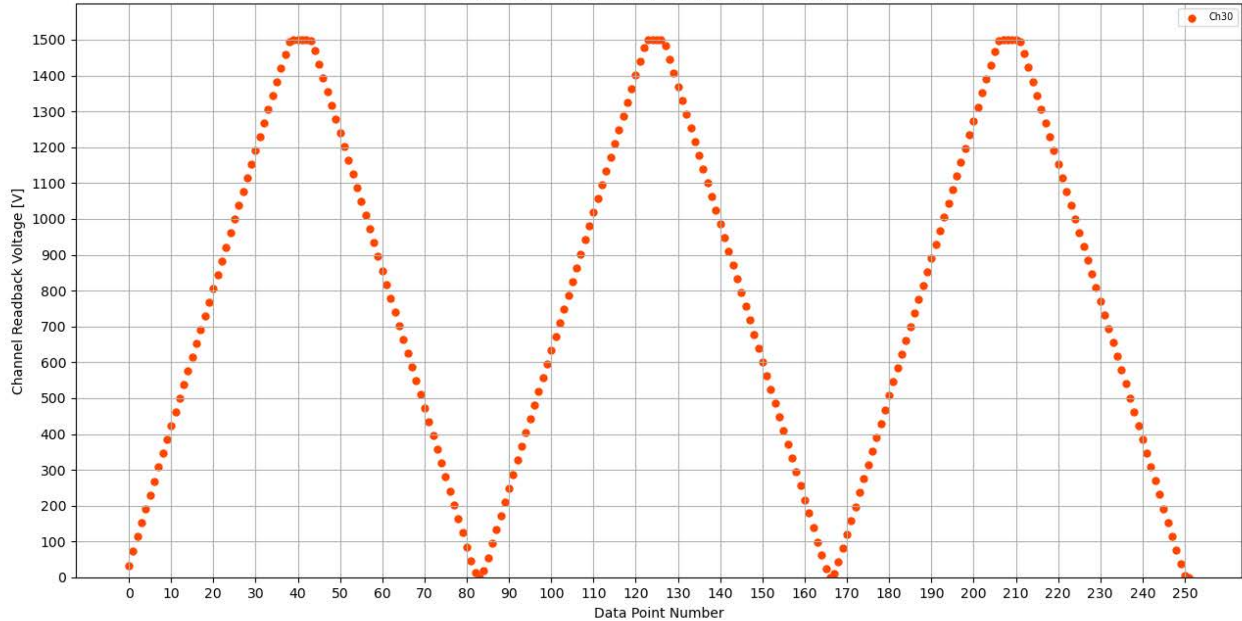
Voltage Ramp Test (Python) Bd #350, Slot #13, Ch #30
