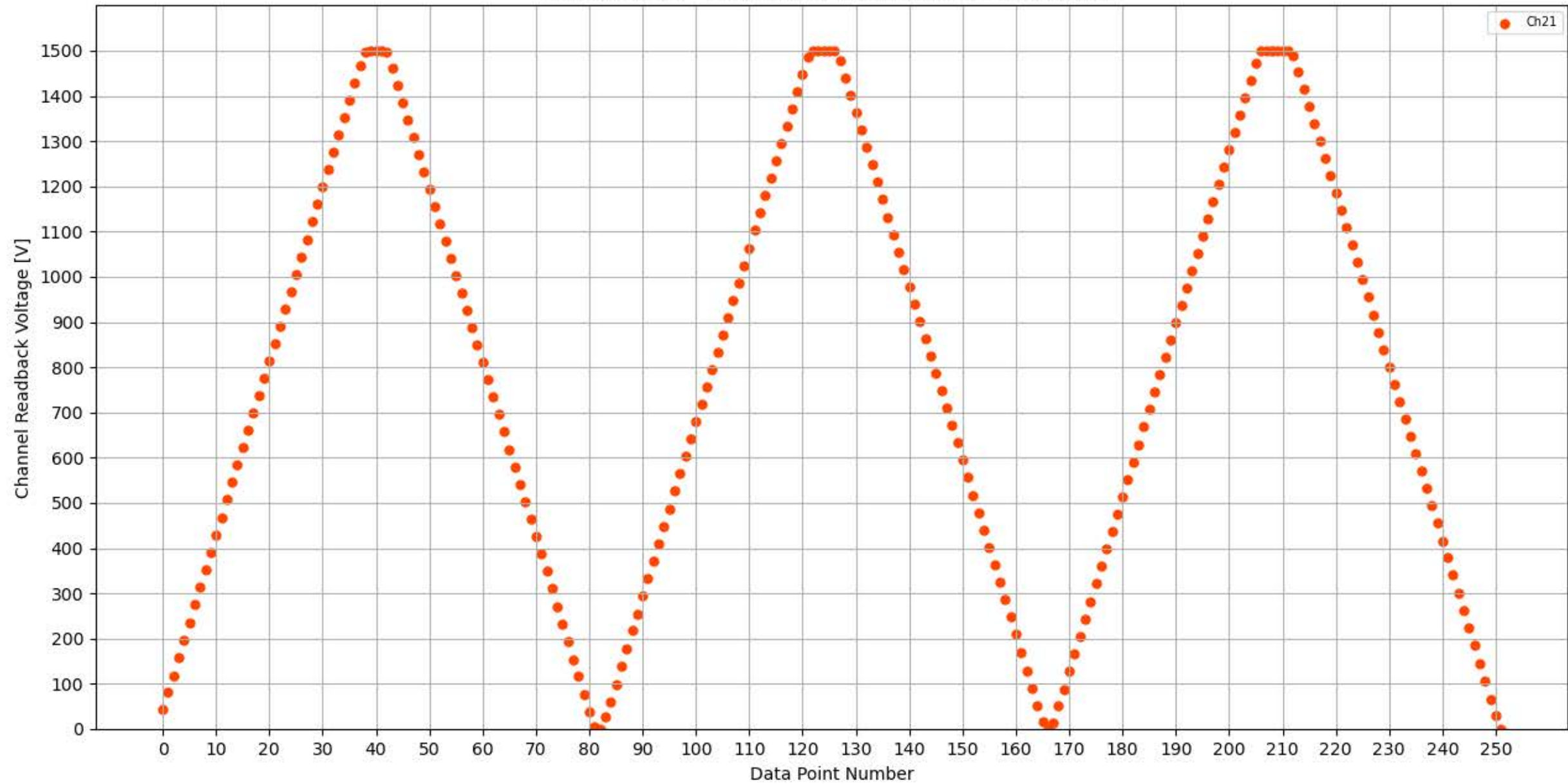
Voltage Ramp Test (Python) Bd #350, Slot #13, Ch #21
