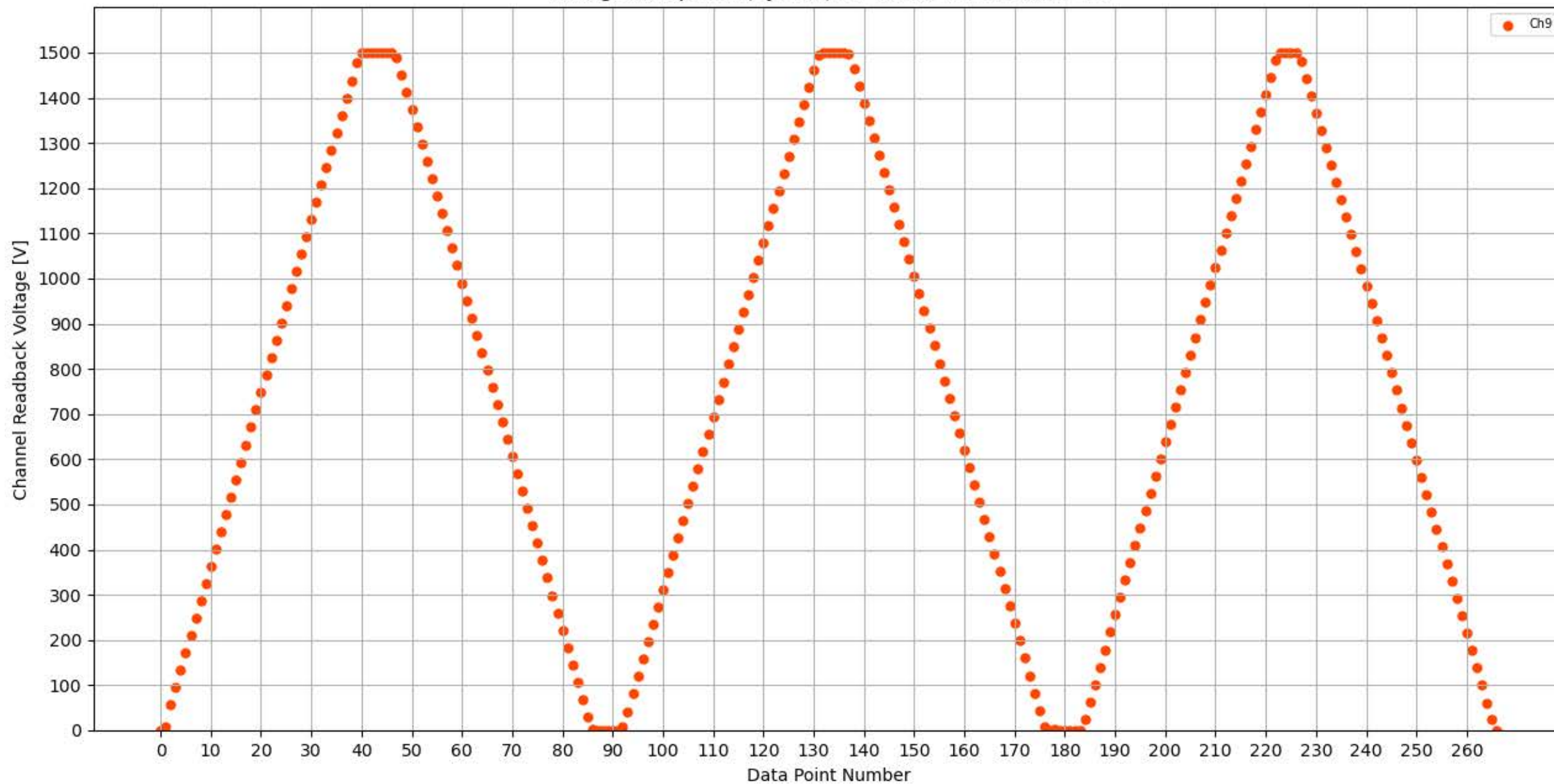
Voltage Ramp Test (Python) Bd #350, Slot #13, Ch #9
