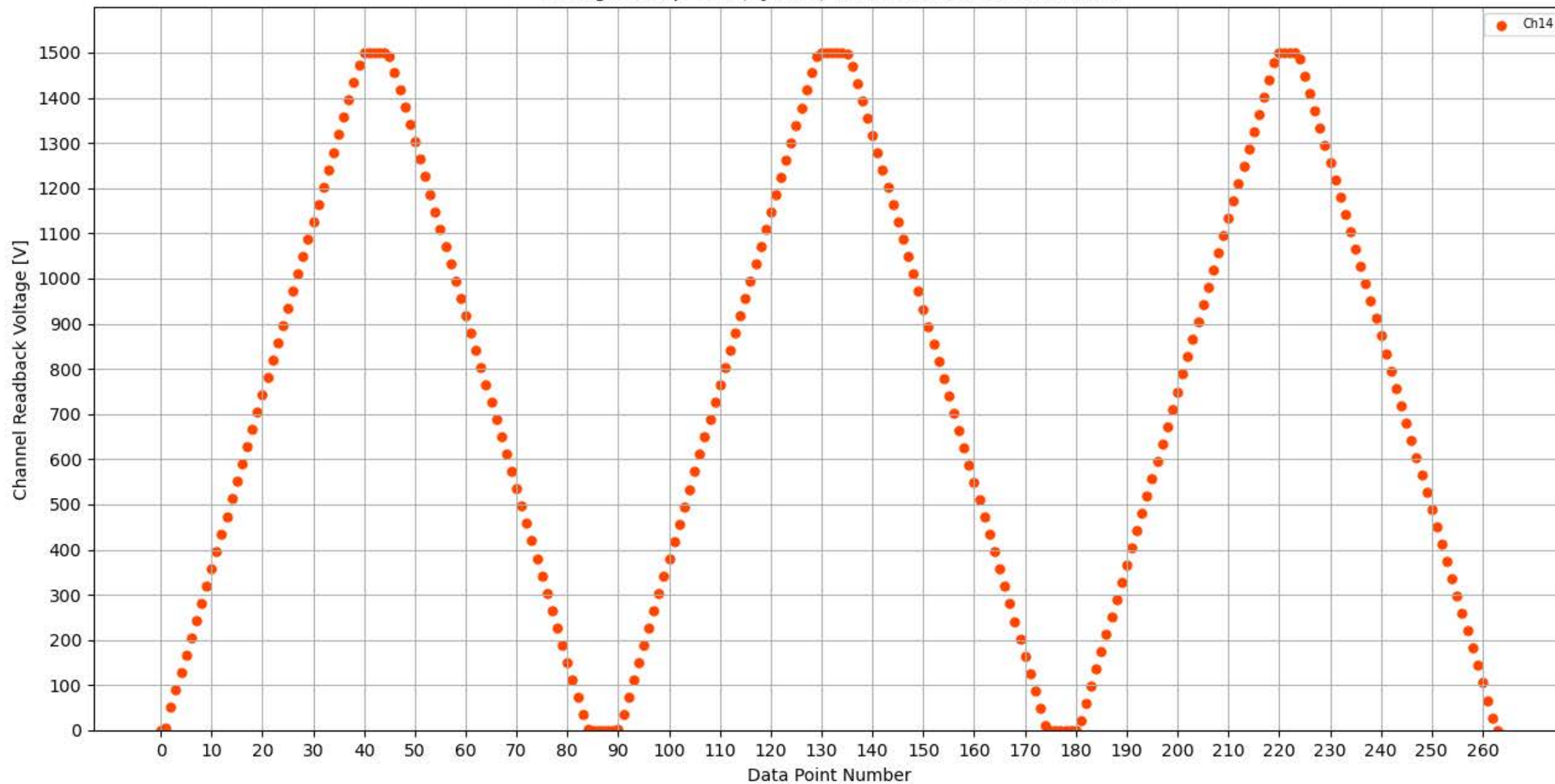
Voltage Ramp Test (Python) Bd #350, Slot #13, Ch #14
