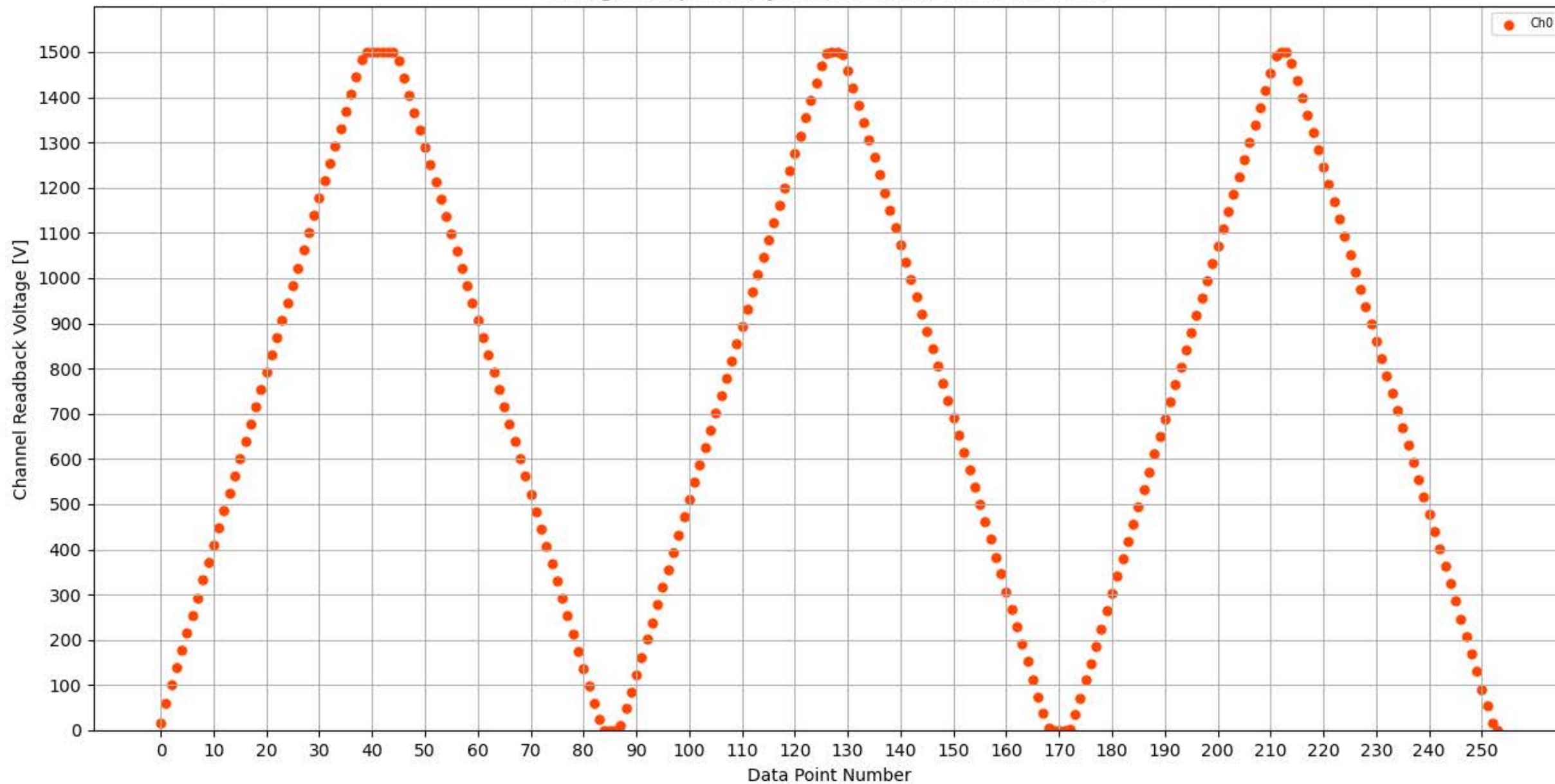
Voltage Ramp Test (Python) Bd #350, Slot #13, Ch #0
