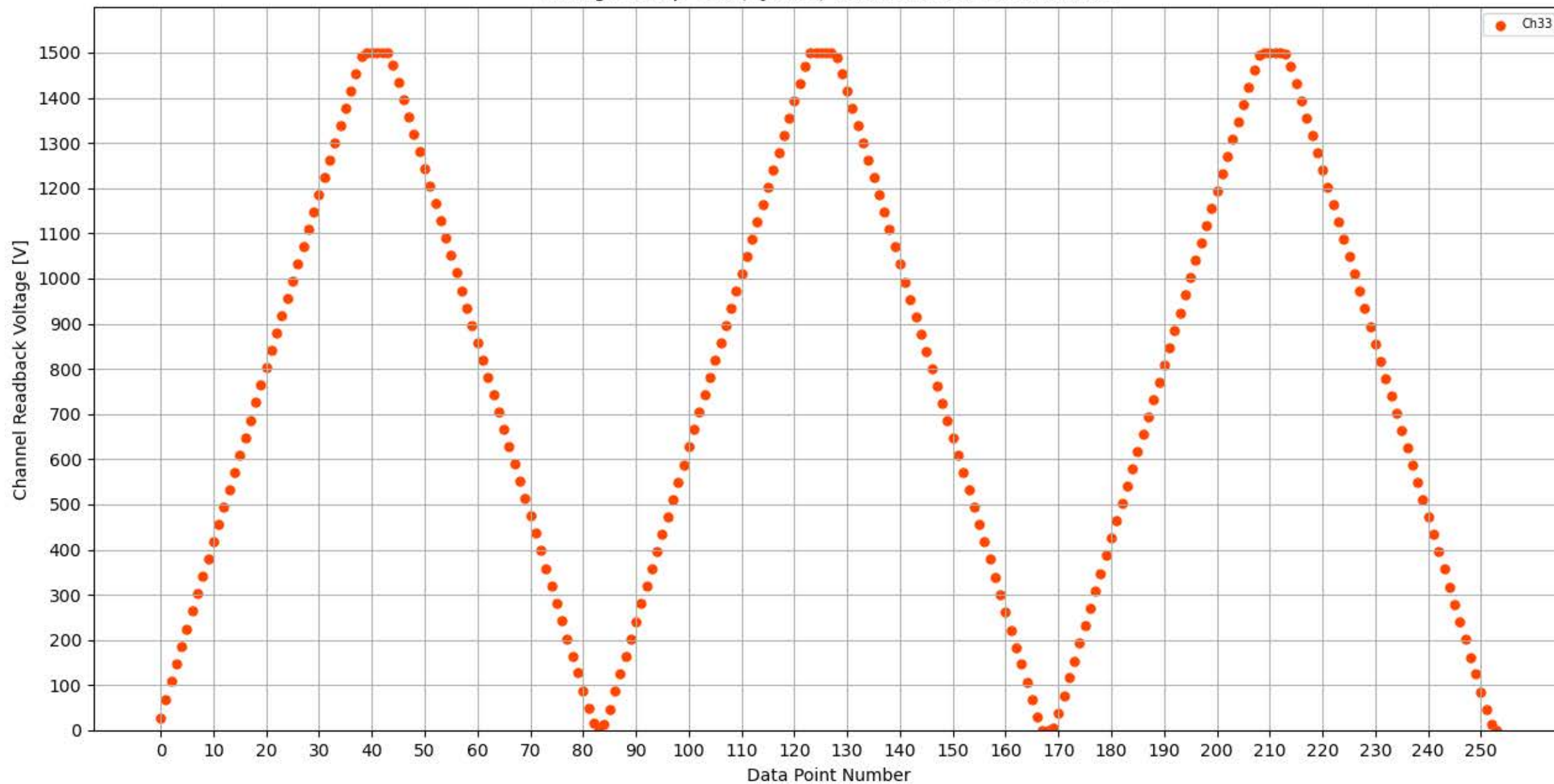
Voltage Ramp Test (Python) Bd #350, Slot #13, Ch #33
