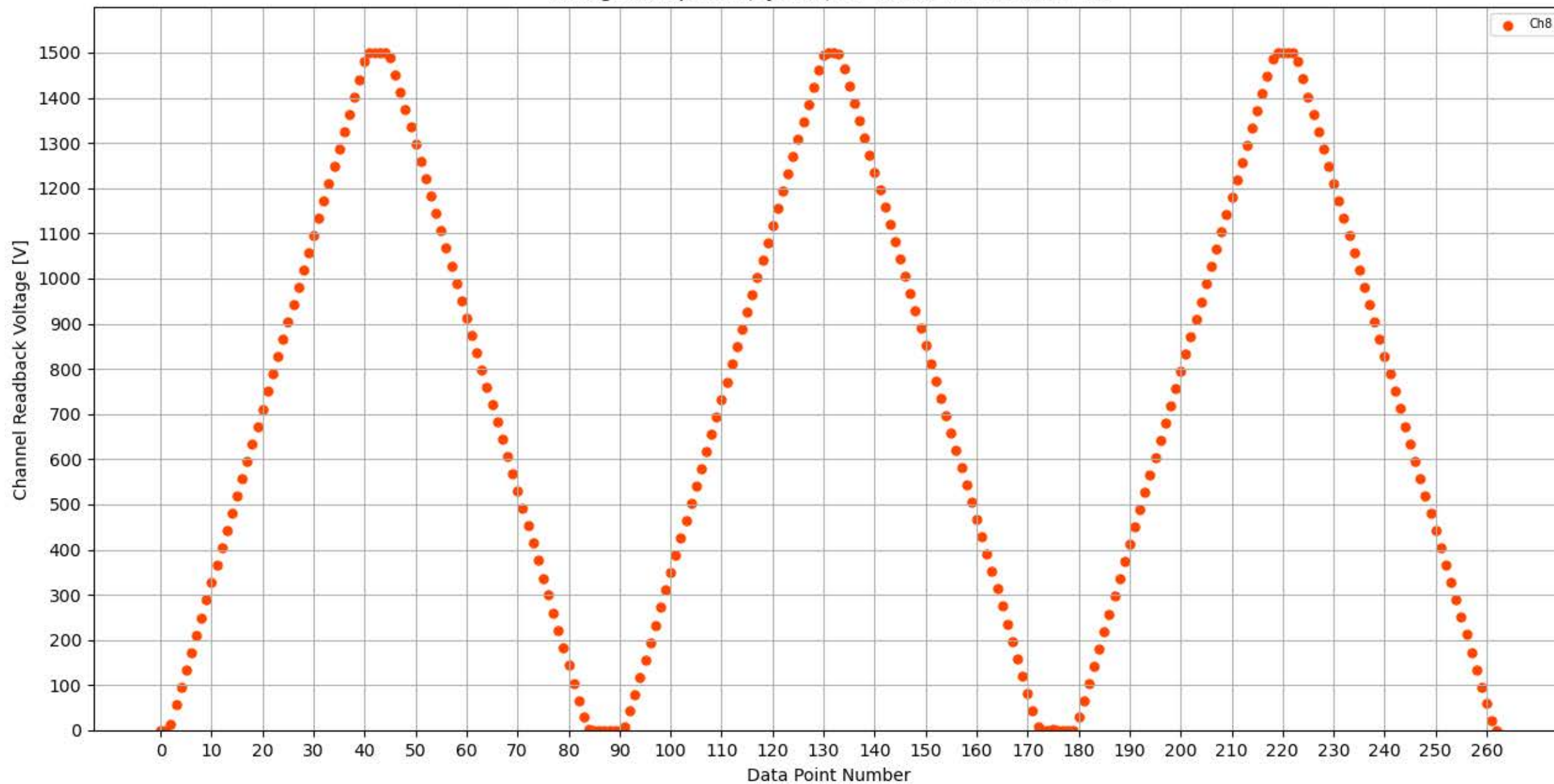
Voltage Ramp Test (Python) Bd #350, Slot #13, Ch #8
