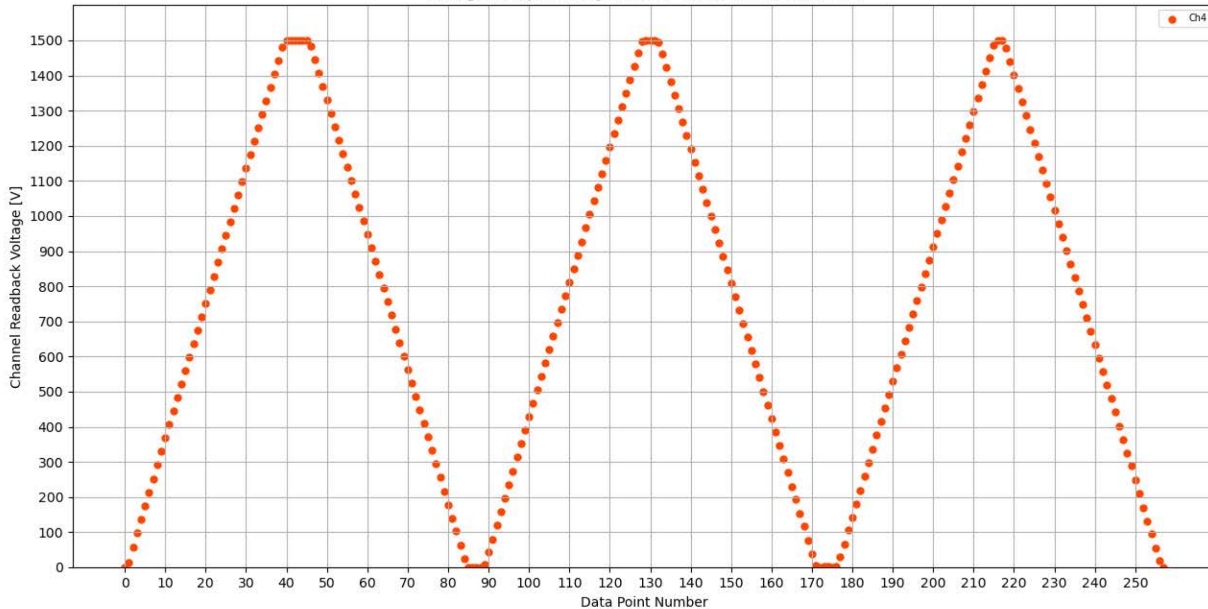
Voltage Ramp Test (Python) Bd #350, Slot #13, Ch #4
