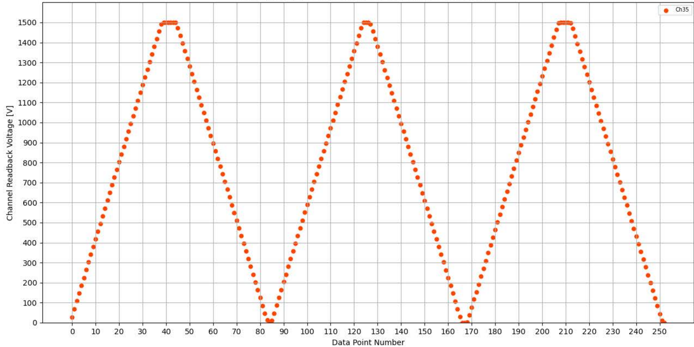
Voltage Ramp Test (Python) Bd #350, Slot #13, Ch #35
