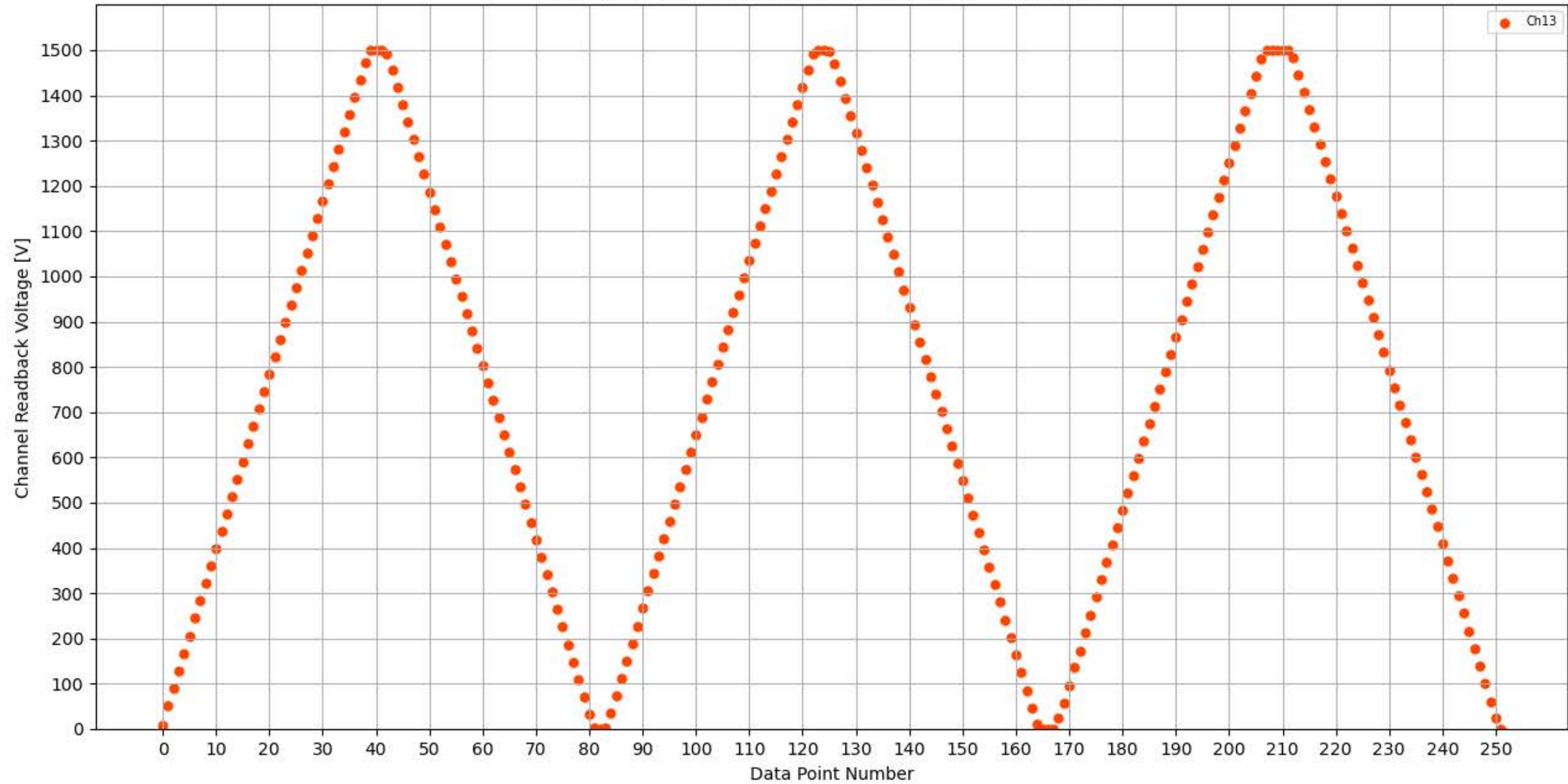
Voltage Ramp Test (Python) Bd #350, Slot #13, Ch #13
