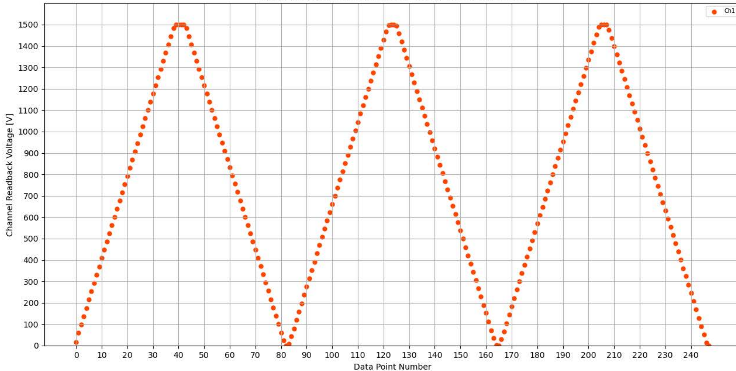
Voltage Ramp Test (Python) Bd #350, Slot #13, Ch #1
