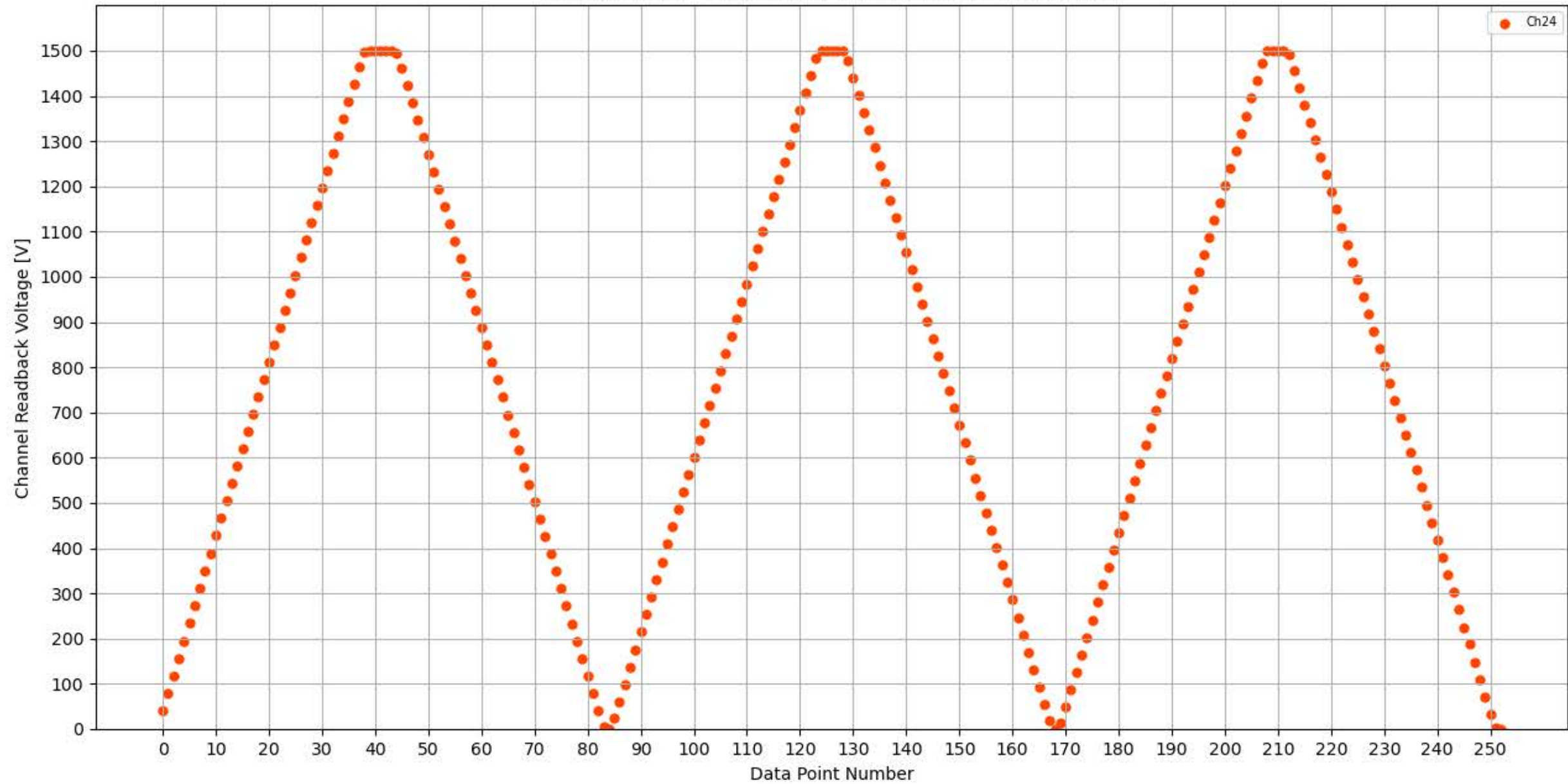
Voltage Ramp Test (Python) Bd #350, Slot #13, Ch #24
