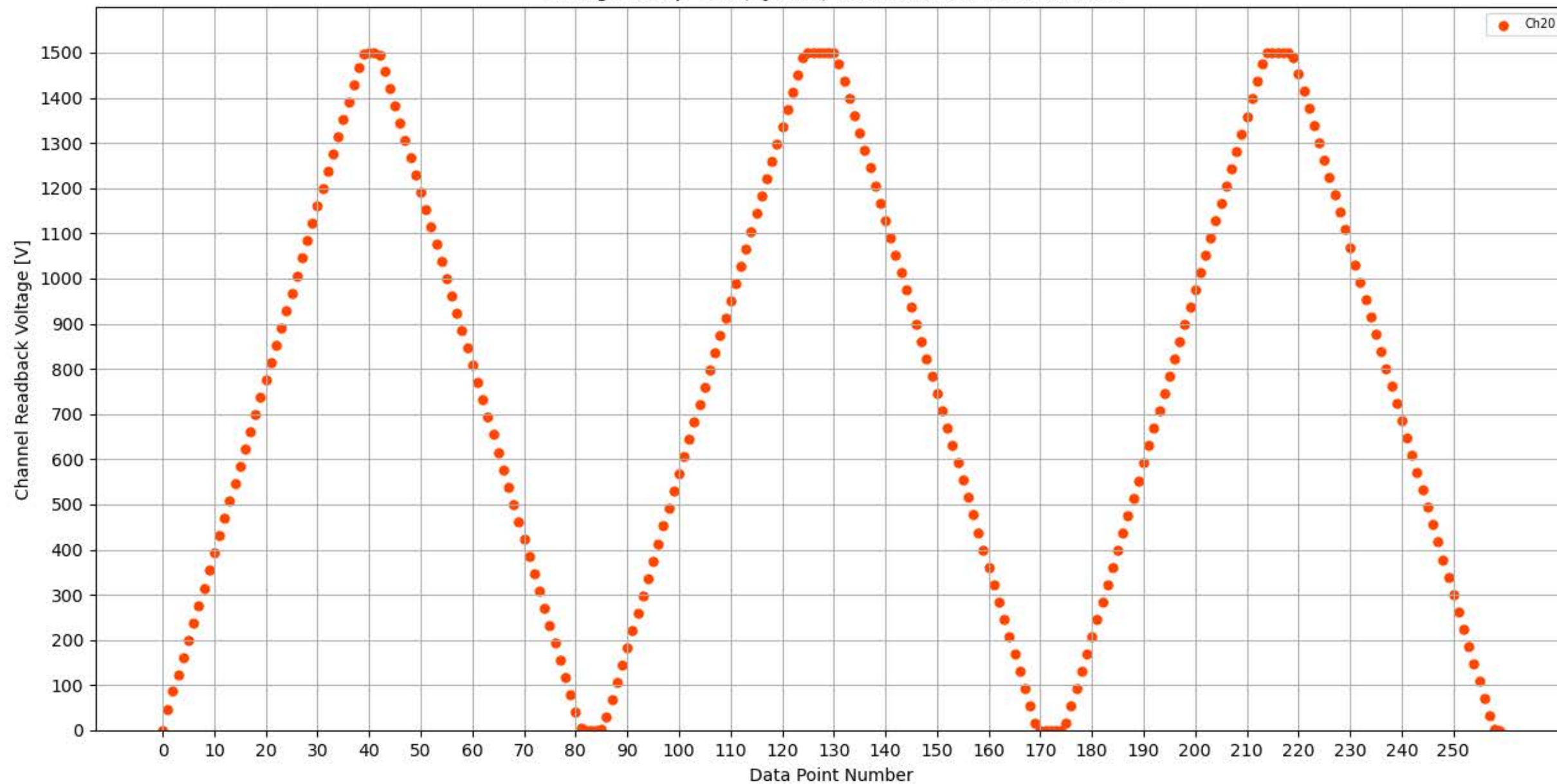
Voltage Ramp Test (Python) Bd #350, Slot #13, Ch #20
