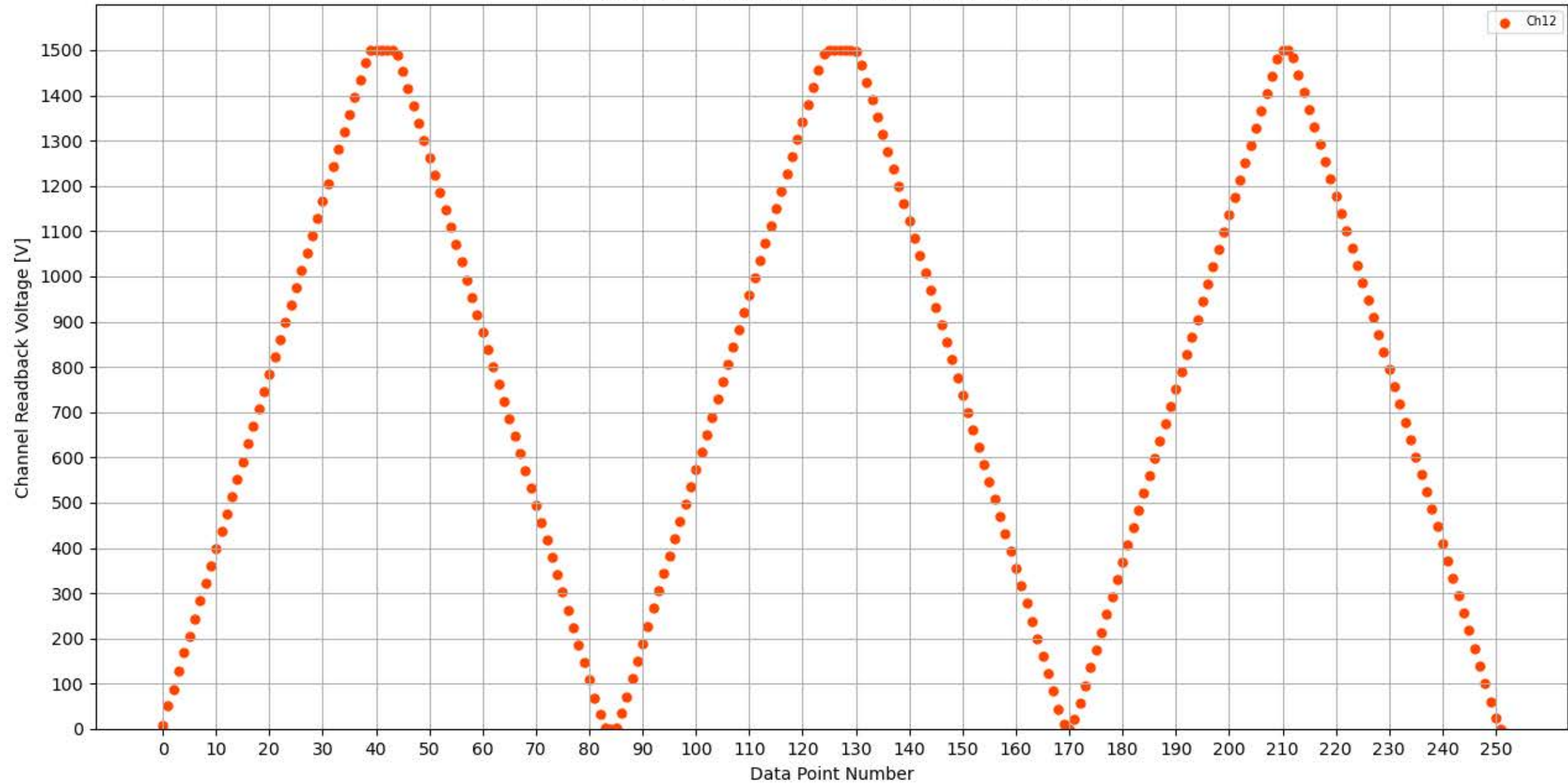
Voltage Ramp Test (Python) Bd #350, Slot #13, Ch #12
