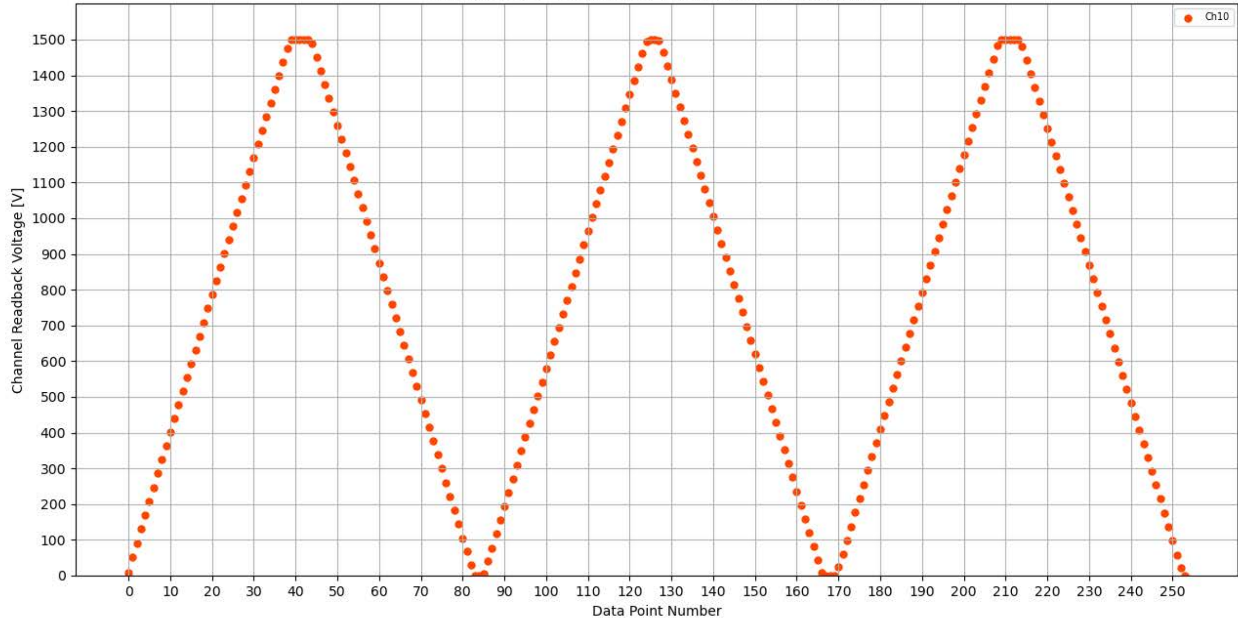
Voltage Ramp Test (Python) Bd #350, Slot #13, Ch #10
