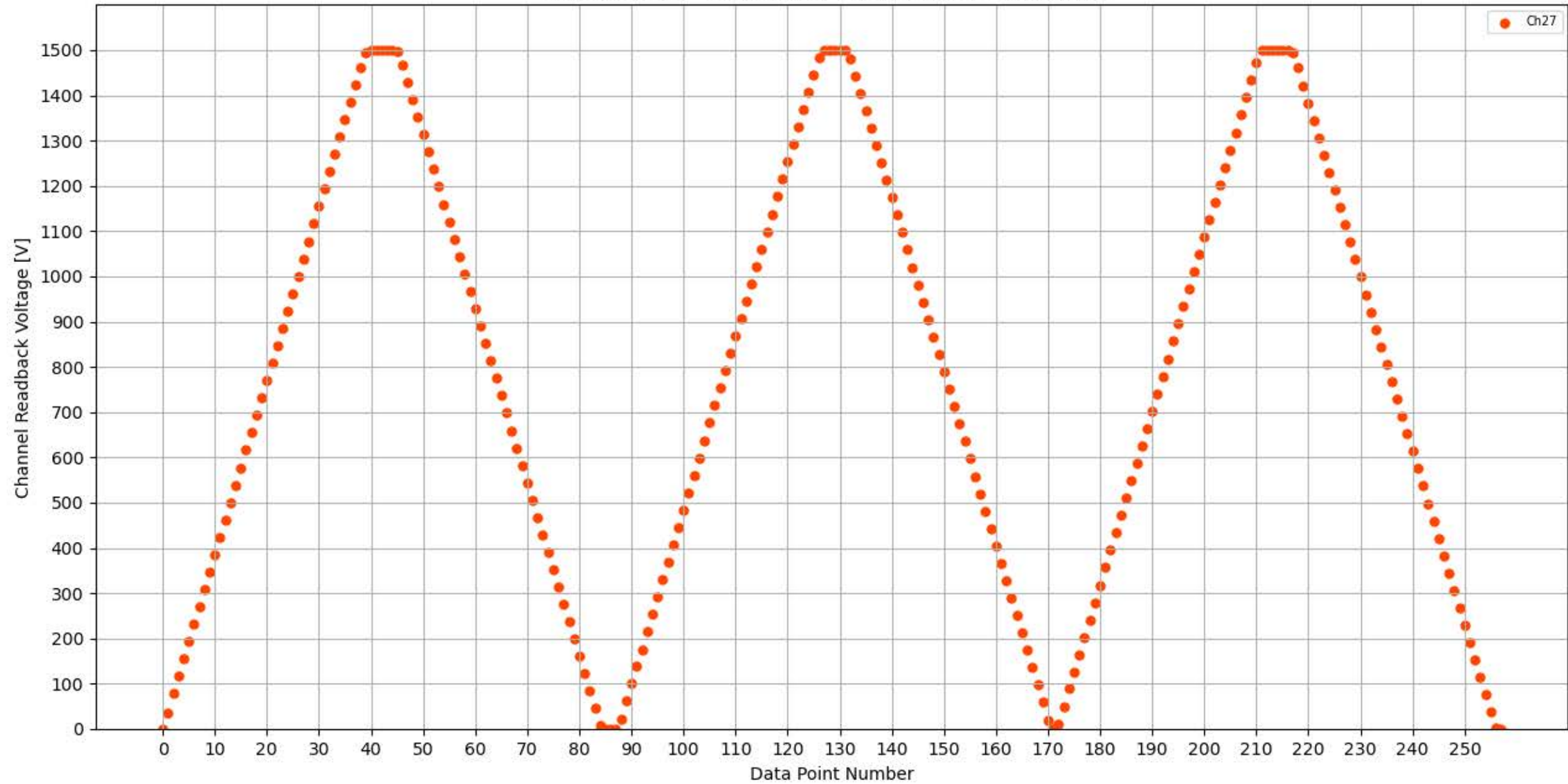
Voltage Ramp Test (Python) Bd #350, Slot #13, Ch #27
