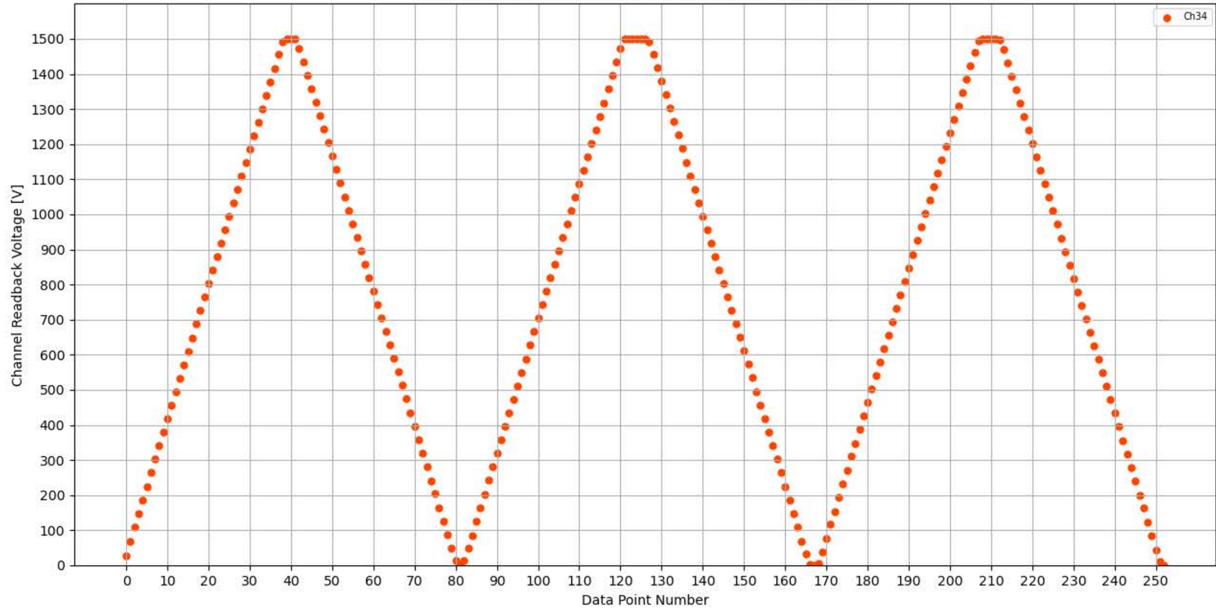
Voltage Ramp Test (Python) Bd #350, Slot #13, Ch #34
