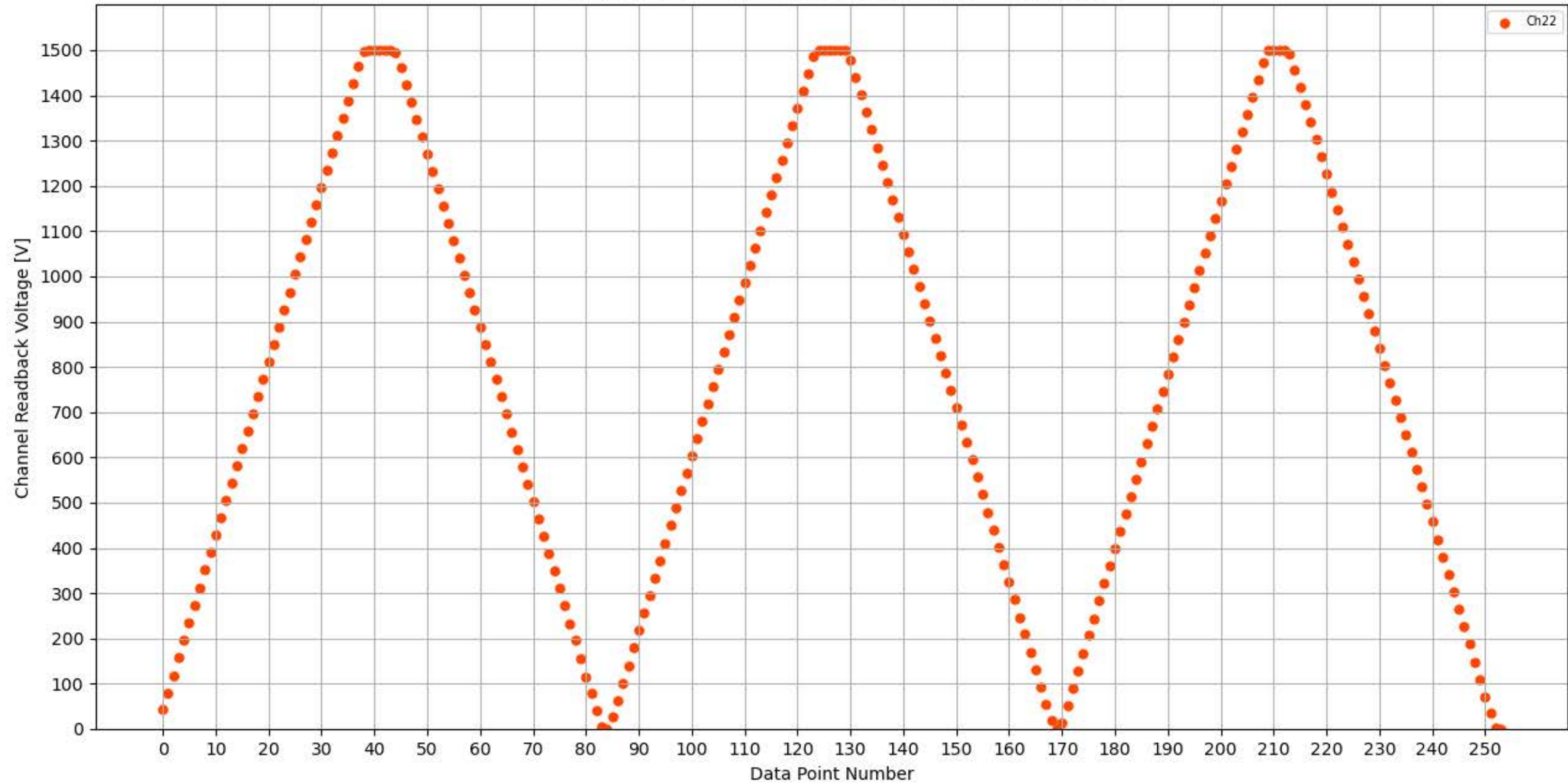
Voltage Ramp Test (Python) Bd #350, Slot #13, Ch #22
